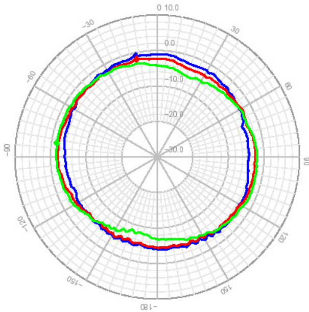
Figure 4 -XM antenna radiation pattern along the horizon (TER performance)
