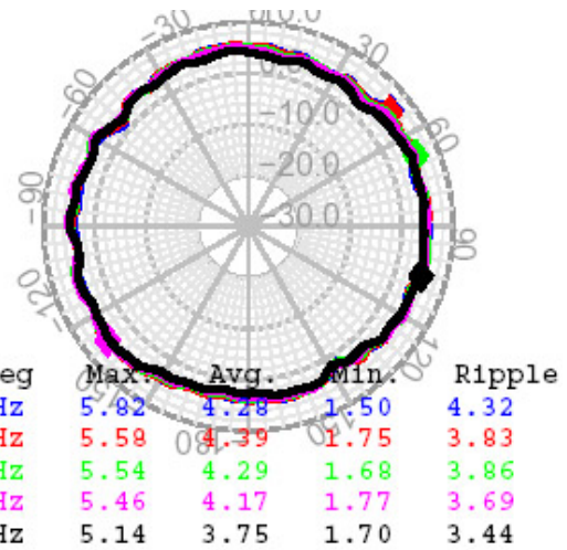
Figure 7 -XM antenna gain at 45-deg elevation angle (vehicle roof)
