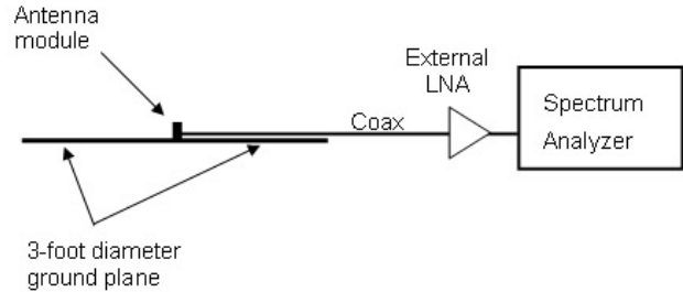
Figure 9b -Y-Factor measurement setup ( P_{cold} )
