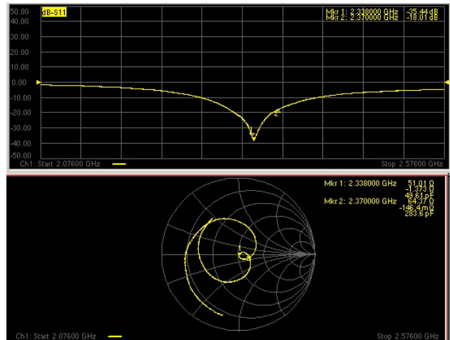
Figure 3-SDARS antenna S11 response
