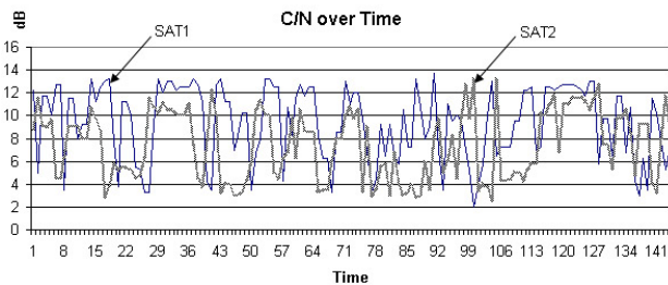
Figure 11- Driving test results corresponding to XM SAT1 and XM SAT 2
