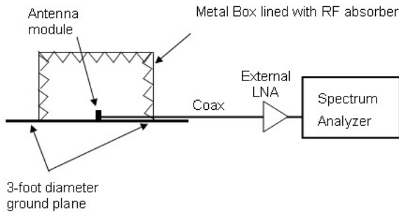
Figure 9a -Y-Factor measurement setup ( P_{hot} )
