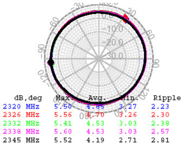
Figure 6 -XM antenna gain at 45-deg elevation angle (ground plane)
