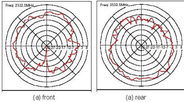
Figure 8 -SDARS antenna gain inside vehicle (25-degree elevation angle)
